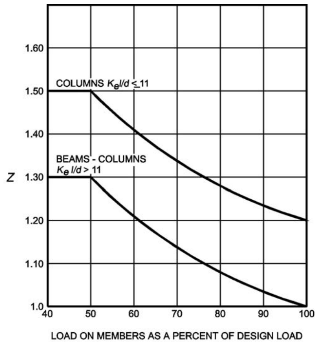
FIGURE 721.6.3(1) LOAD FIGURE
