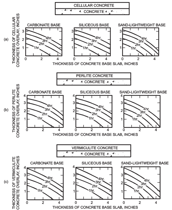
FIGURE 721.2.2.3(1) FIRE-RESISTANCE RATINGS FOR CONCRETE ROOF ASSEMBLIES
